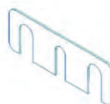
KG-FG models
